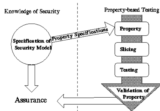
Figure 6: PBT Model
