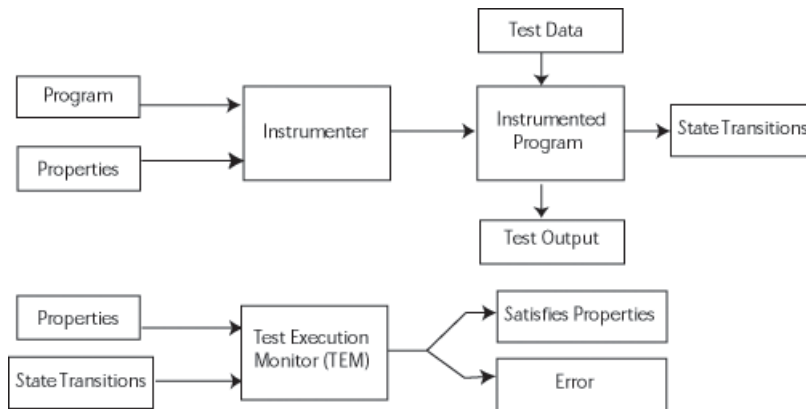
Figure 5: PBT Process
