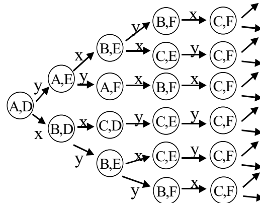
Figure 3: State Space
